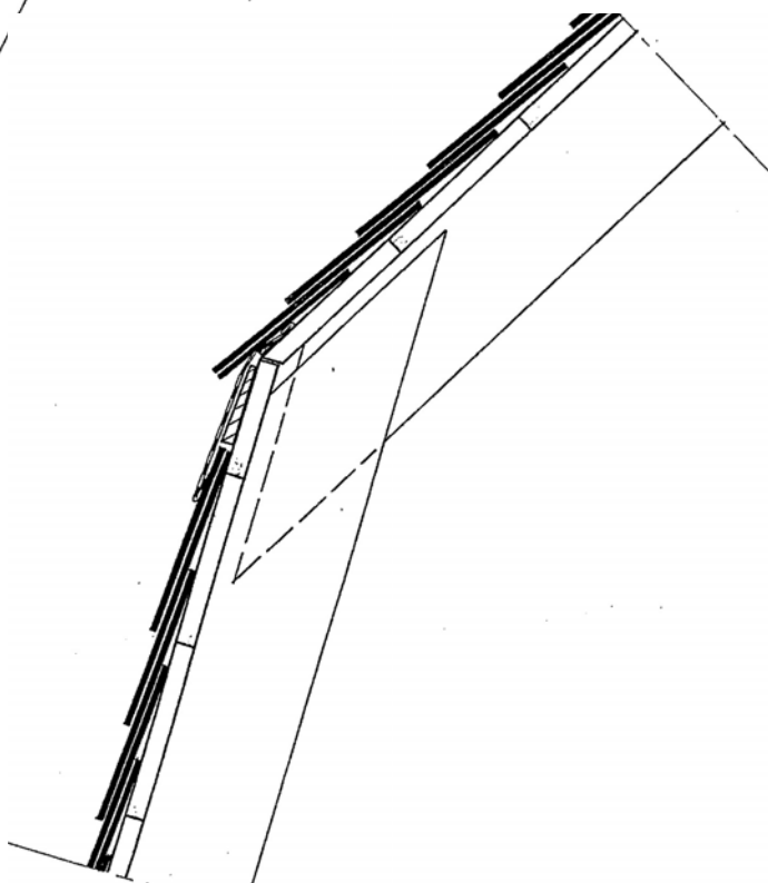
Detail 14b. Knik in dak (uitwendig)
